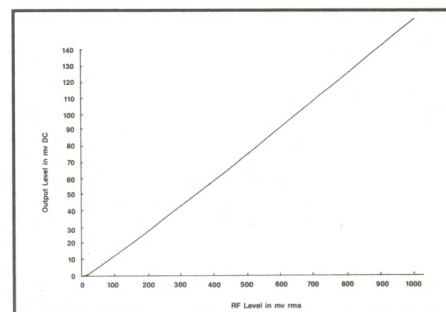
Figure 2. Envelope detector response for the circuit of Figure 1.
