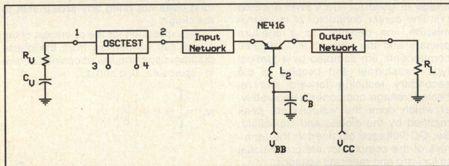
Figure 4. Oscillator schematic showing the use of the OSCTEST simulation element.
