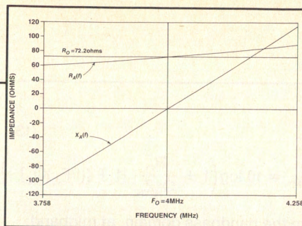
Figure 11. Impedance versus frequency for a 4 MHz half-wave dipole in free space.
