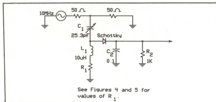
Figure 3. Low level envelope detector with lower L/C ratio to illustrate the effect of R_1 .
