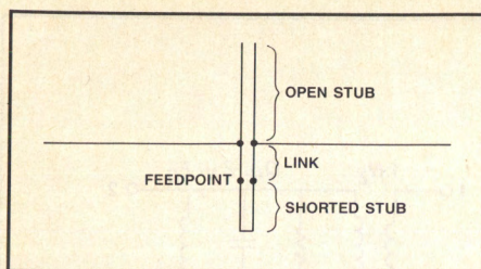
Figure 14. Half-wave dipole employing a quarter-wave matching network.
