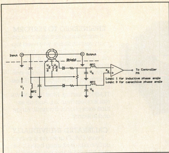
Figure 3. Schematic diagram of the phase angle sensor.
