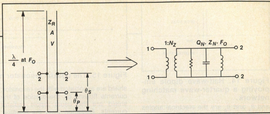
Figure 13. The quarter-wave resonator/transformer.
