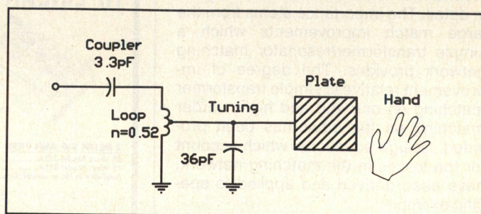
Figure 2. Plate antenna with loop.
