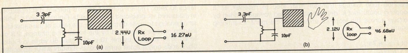
Figure 6. Receiver voltage with (a) tuned loop and plate; (b) tuned loop, plate and hand.
