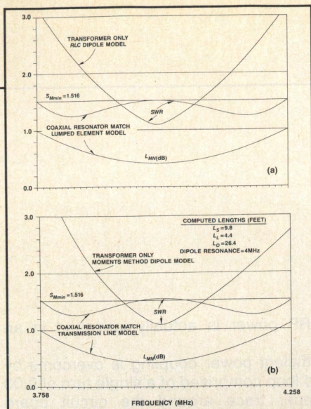
Figure 16. SWR and matching loss for coaxial resonator match example. (a) RLC dipole and lumped element matching, (b) moments method dipole and transmission line matching model.
