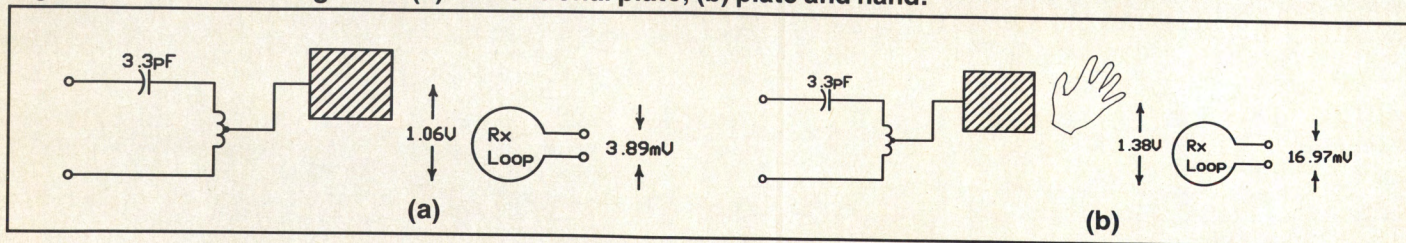
Figure 5. Receiver voltage with (a) plate and loop; (b) loop, plate and hand.
