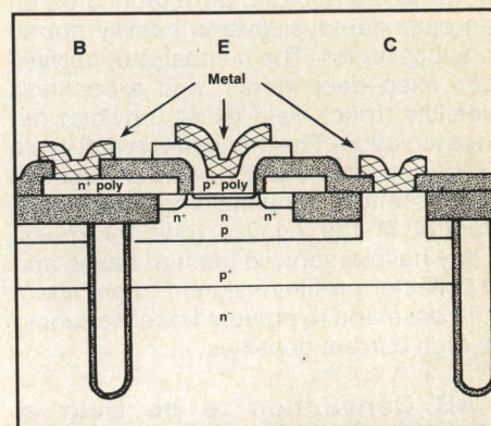
Schematic cross section of the PNP transistor.
