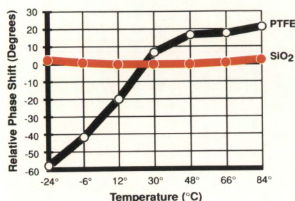
PHASE SHIFT vs. TEMPERATURE 0.141" Dia. Cable @ 5.5 GHz
