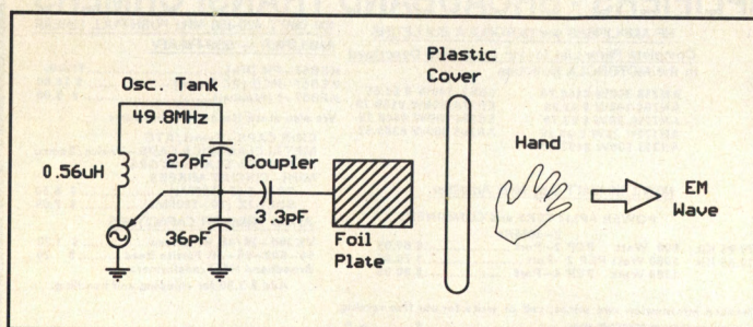
Figure 1. Conventional hand coupled plate.
