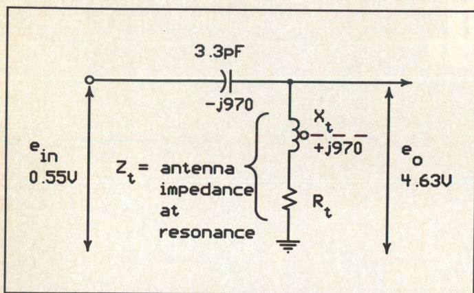
Figure 3. Impedance of loop and plate.
