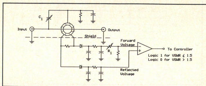
Figure 2. Schematic diagram of the VSWR sensor.
