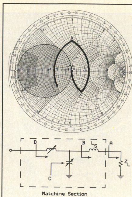
Figure 9. Shaded area will be transformed to the shaded region of Figure 8 by using L_s (0.3uH) transformation inductance. The network configuration is used. Example of a matching path in that region. B to D path as shown in Figure 8.
