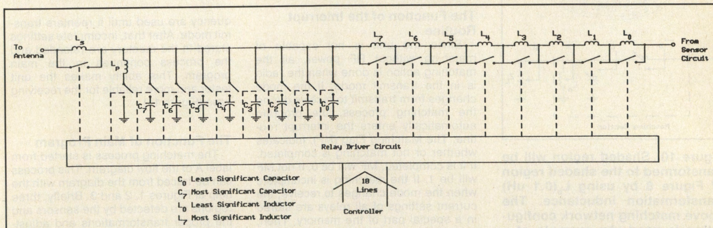
Figure 7. The matching network.
