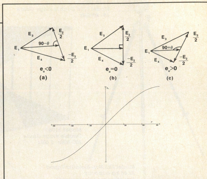
Figure 4. Voltage vector diagram a) e_o < 0 ; b) e_o = 0 ; c) e_o > 0 ; d) output voltage versus phase variation of phase angle sensor.
