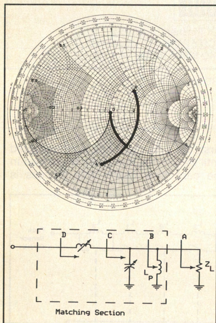
Figure 10. Shaded region will be transformed to the shaded region of Figure 8 by using L_p (0.1 uH) transformation inductance. The above matching network configuration is used. An example of a matching path in that region.
