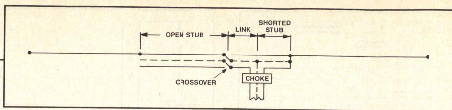
Figure 15. The coaxial resonator match.
