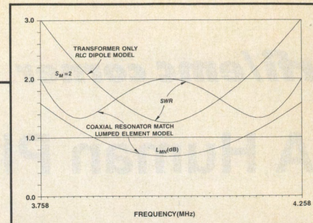
Figure 18. SWR and matching network loss for the "-" root of equation 20.
