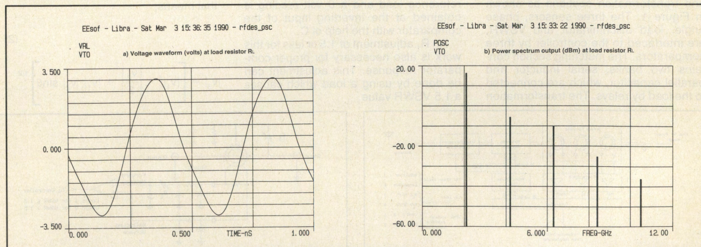
Figure 5. Oscillator output voltage and power spectrum simulated by Libra for oscillation at f = 2.1 GHz.
