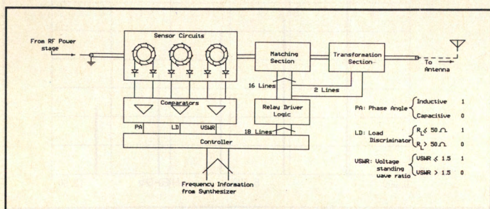
Figure 1. Block diagram of antenna matching unit.
