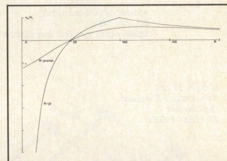
Figure 6. Output voltage versus resistance variation of load discriminator.
