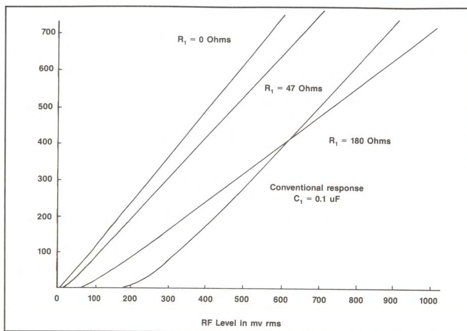
Figure 5. Envelope detector response for 3 values of R_1 .
