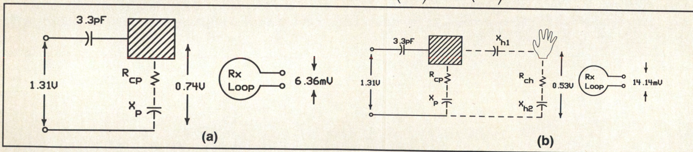
Figure 4. Receiver voltage with (a)conventional plate; (b) plate and hand.
